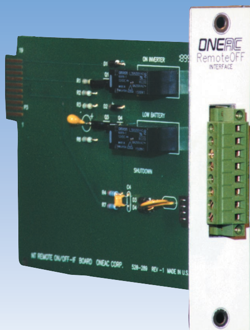
Providing Remote Off Control for ON Series UPSs
